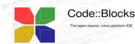
Gambar 2. Code::Blocks
