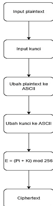
Gambar 2. Proses enkripsi beaufort cipher
