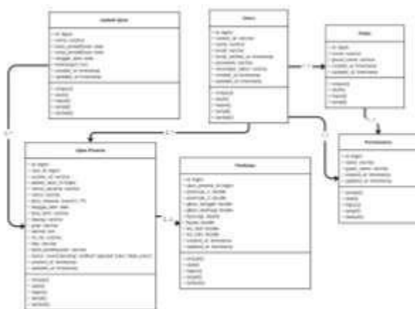
Gambar 2.7 Class Diagram
